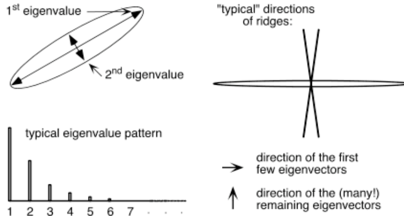
Figure 10. Upper left: Contour line of a bivariate distribution, supposedly of mutational steps. The lengths of the two axes of the ellipse, called principal components, are proportional to the square root of the eigenvalues of the mutational covariance matrix. Lower left: Typical eigenvalue pattern found for large empirical covariance matrices. Right: The mutation distribution will rarely be fully aligned with the fitness ridges. If in a high dimensional fitness landscape one takes one's perspective from the mutation distribution and looks at the orientation of the ridges relative to the first few principal axes of this the mutation distribution, then, when the number of the dimensions of the trait space is very large and the ridge has a relatively low dimensional top, the ridge will typically extend in a direction of relatively small mutational variation.
