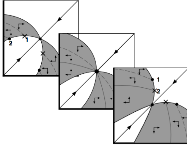
Figure 8. Three TEPs corresponding to a bifurcation of an ESS to a branching point. In this case the adaptive tracking of the ESS stops due to a change in character of the ess. In the fossil record this scenario would correspond to a punctuation event that starts with speciation.
