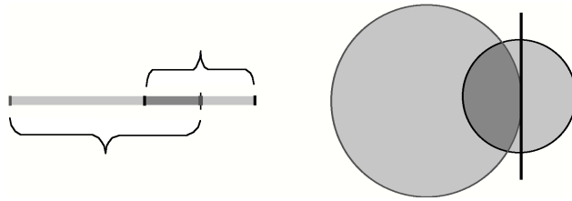
Figure 9. Left: Two balls in \mathbb{R}^1 , with the centre of the smaller ball on the boundary of the larger ball. The ratio of the volume of their intersection to the volume of the smaller ball is 1/2 . Right: A similar configuration in \mathbb{R}^2 . The volume of the intersection is now a smaller fraction of the volume of the smaller ball. For similar configurations in \mathbb{R}^n this fraction quickly decreases to zero for larger n . Now think of the larger ball as the part above sea level of a fitness hill and of the smaller ball as a mutation distribution. Clearly the fraction of favourable mutants will go to zero with n .
