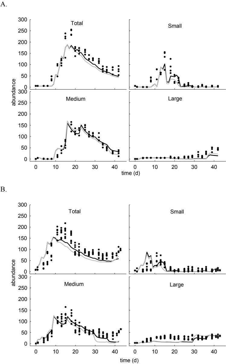
Fig. S3 Comparison of starvation-recovery assumptions at the high food population level for the lowN (A) and lowNA (B) experiments. The grey line show the average of 100 model simulations when individuals feed at a rate proportional to their current length, while the black line represents the average of 100 model simulations when individuals feed at a rate proportional to their maximum length attained.
