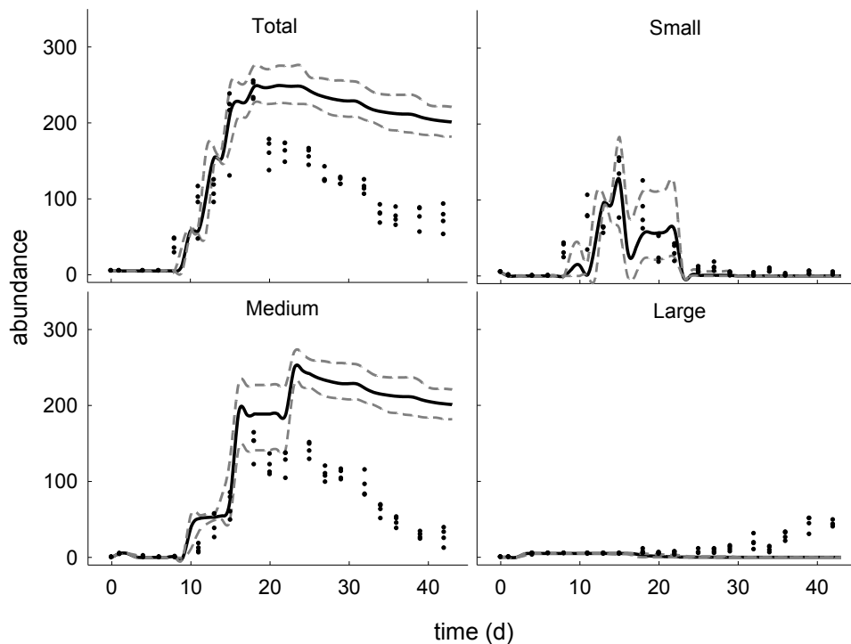
Fig. 3 Comparison of data and DEB-IBM predictions at the population level for the lowN experiment. Experiments were initiated with 5 neonates in a 900ml beaker, and 0.5mgC was added per day. Simulations with DEB-IBM replicated the experimental conditions. Figures show the mean (thick black line) and max and min (dashed grey lines) of 50 simulations. Simulations for the lowNA and highNA experiments are shown in figure S1.
