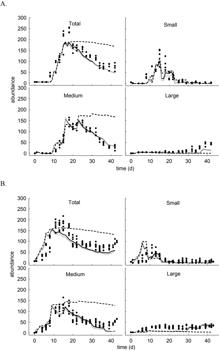
Fig. S2 Comparison of the performance of three starvation submodels with data from the lowN (A) and lowNA (B) experiments. In each of the three models, a 1-parameter food-dependent mortality submodel, was applied, but models differed in that it was either applied only to juveniles (black solid), only adults (black dashed), or all Daphnia (grey solid).
