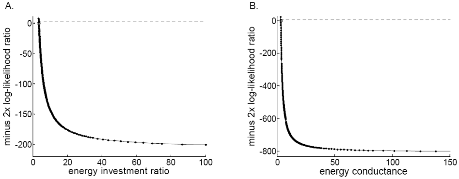
Fig. B1 Confidence intervals for the energy investment ratio, g (A) and energy conductance, \dot{v} (B) using the profile likelihoods method (Meeker and Escobar 1995). For both g and \dot{v} the model fit continued to improve at a decreasing rate as their values increased.
