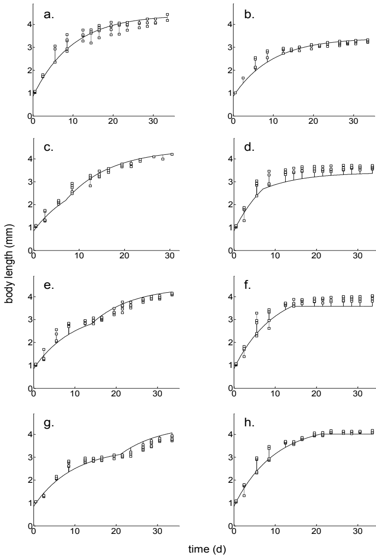
Fig. 2 Observed (open squares) and predicted (lines) body sizes over time for Daphnia magna at 20°C fed either a constant daily dose of green algae at either a high (a.) or low (b.) density, or switched from one feeding level to another (c.-h.). Panels c., g., and e. show the scenario where Daphnia were switched from the low food concentration to the high food concentration at 7, 14, or 21 days after birth, respectively. Panels d., f., h., show the scenario where Daphnia were initially feed at the high daily food density and switched to the low food density on days 7, 14, or 21 respectively. The model predictions used parameter values from Table 1, in Chapter 3. Only panels a. and b. were used to estimate f for each food concentration.
