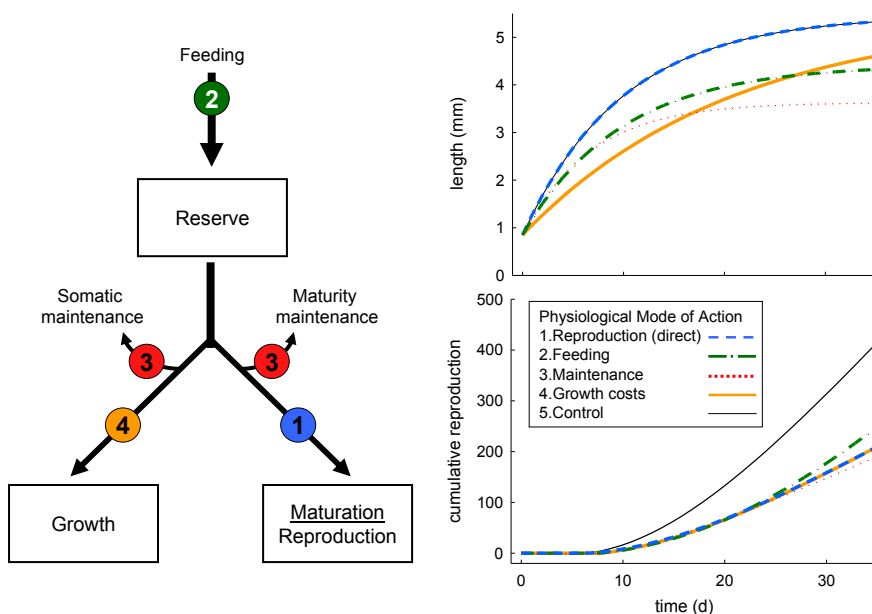
Fig. 1 The left panel shows a schematic diagram of energy flow in a DEB model. The parameter values for a species and the state of the environment (characterized here by food density) determine the magnitude of the energy fluxes into, within, and out of the organism. These fluxes specify the change over time of measurable quantities such as growth or reproductive output. Stressors are modelled in DEB as changes in the value of one or more parameters thereby modifying one or more of the energetic fluxes leading to different patterns in growth and or reproduction. The pattern of the stressed life history output depends on the physiological mode of action (PMoA). In the right panel, the black line shows the predicted body size and cumulative reproduction for Daphnia magna in ad libitum feeding conditions over the course of 35 days, using the DEB model parameterized for Daphnia (Martin et al., in press). For all other lines in the right panel we calculated the needed stress level for each PMoA shown in the left panel that would result in 50 % reduction in reproduction in a 21 day Daphnia reproduction test. Then, for each PMoA in the left panel, we used the stressed values for a parameter to simulate growth and reproduction under the same conditions as the control to compare the patterns of life-history output predicted by the different PMoAs. The colours of each line in the right panel correspond the PMoA that is simulated from the left panel. The vertical black line represents where the end of a 21 day Daphnia reproduction test would occur and data would be recorded.
