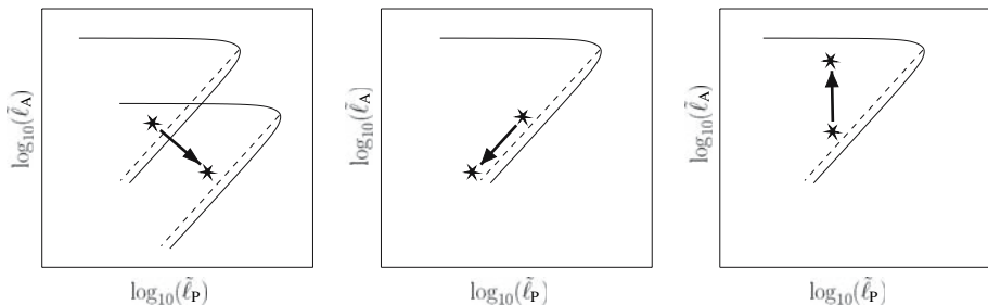
Fig. 6 Three different types of change in evolved predator–prey patterns. Continuous curves delineate the boundaries of the coexistence set, dashed lines show the outcomes of single-trait evolution, and asterisks indicate the evolutionary outcome of two-trait predator evolution when a range of prey types is present. Arrows depict changes in the predator's two adaptive traits \tilde{A} (vertical) and \tilde{P} (horizontal): (a) the expected outcome of evolution in predator body size and predator–prey size ratio is changed, together with the coexistence set; (b) predator body size evolves, while the predator–prey size ratio remains the same; (c) the predator evolves away from the body size and size ratio predicted by single-trait predator evolution
