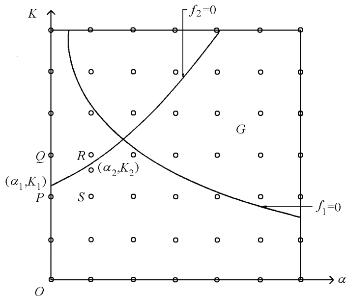
Figure 3: Determination of the zero's of f_1 = 0 and f_2 = 0 .
