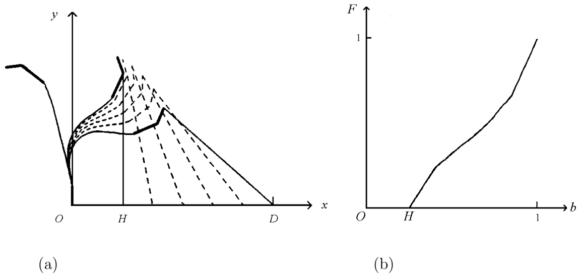
Figure 10: (a) Dimensionless deformation curves of the "Asiatic bow". (b) Dimensionless force-draw curve of the "Asiatic bow".
