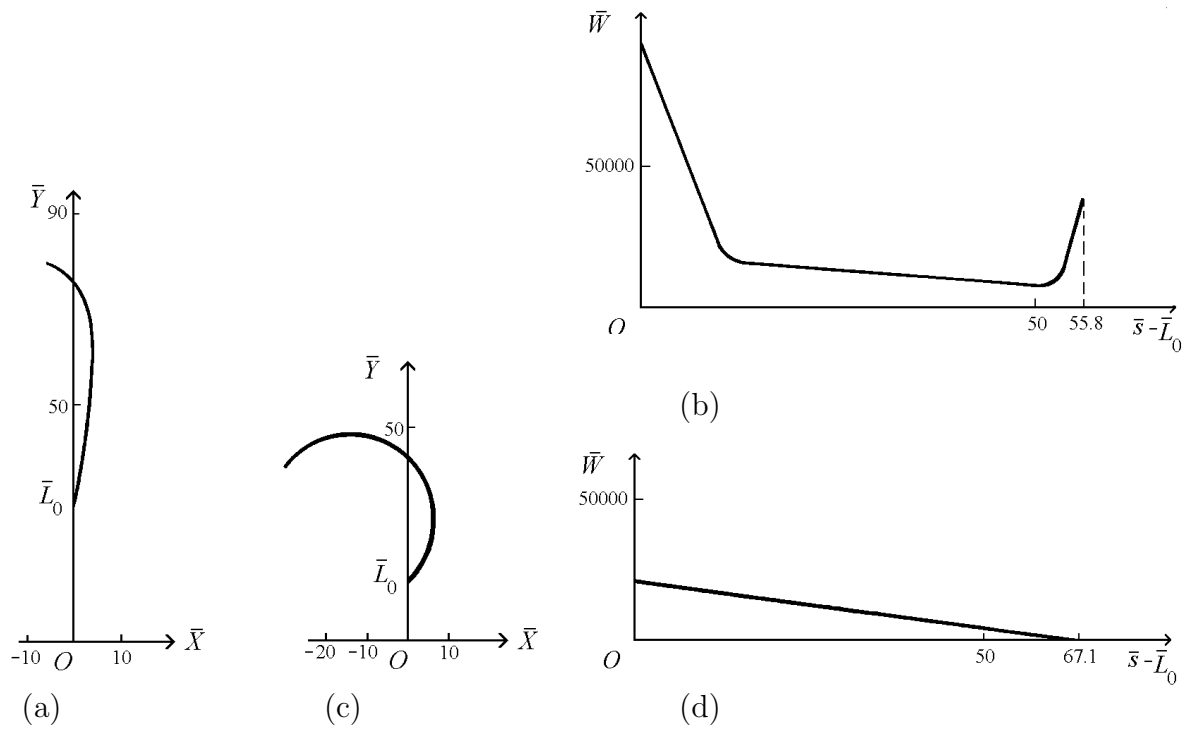
Figure 6: (a), (b) a modern recurve bow B_1 , \theta_0(\bar{s}) and \bar{W}(\bar{s}) , (c), (d) a bow with strong recurve B_2 , \theta_0(\bar{s}) and \bar{W}(\bar{s}) .
