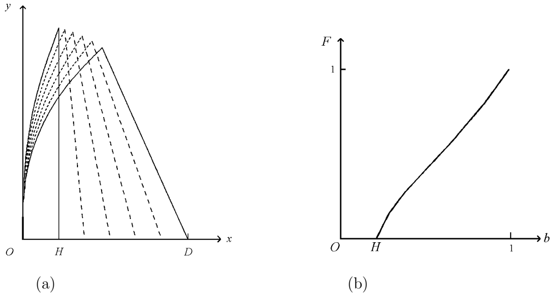
Figure 4: (a) Some shapes of the dimensionless deformations of the H bow. (b) Dimensionless force-draw curve of the H bow.
