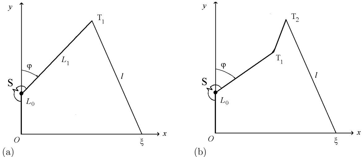
Figure 13: Two bows each with two elastic hinges and rigid limbs.
