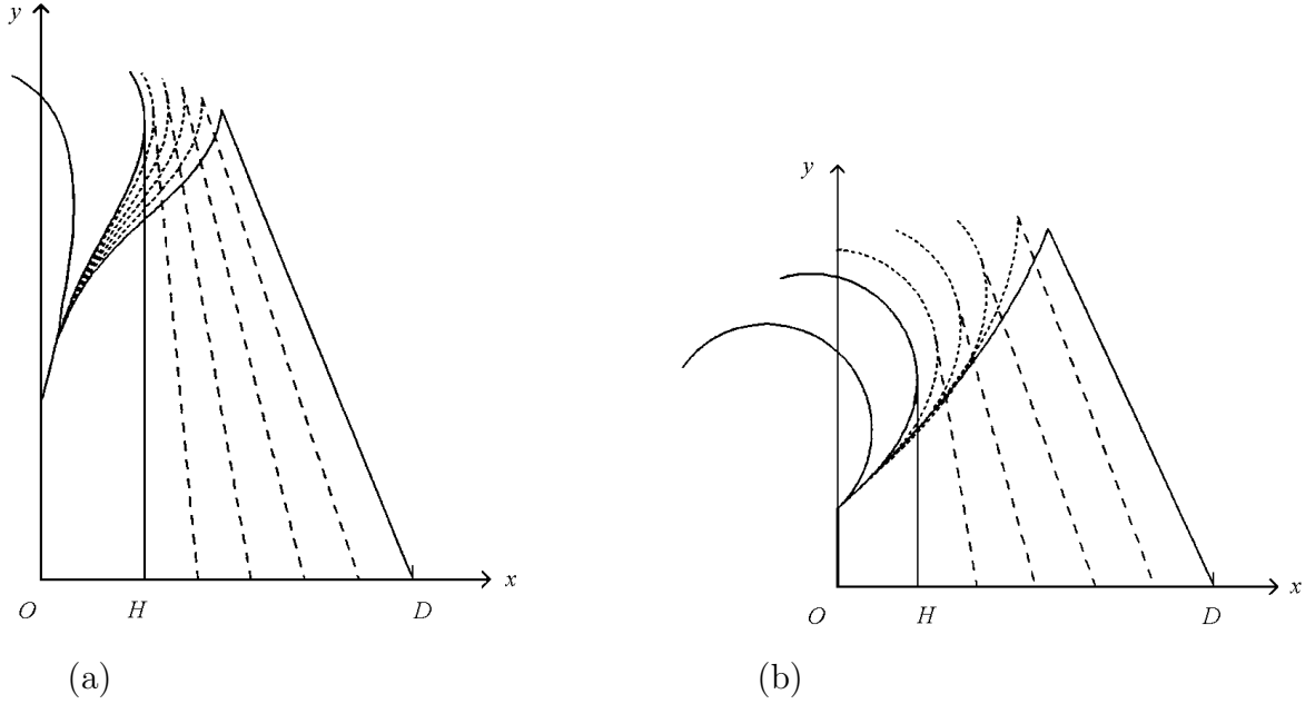
Figure 8: (a) Dimensionless deformations of the B_1 bow. (b) Dimensionless force-draw curve of the B_2 bow.
