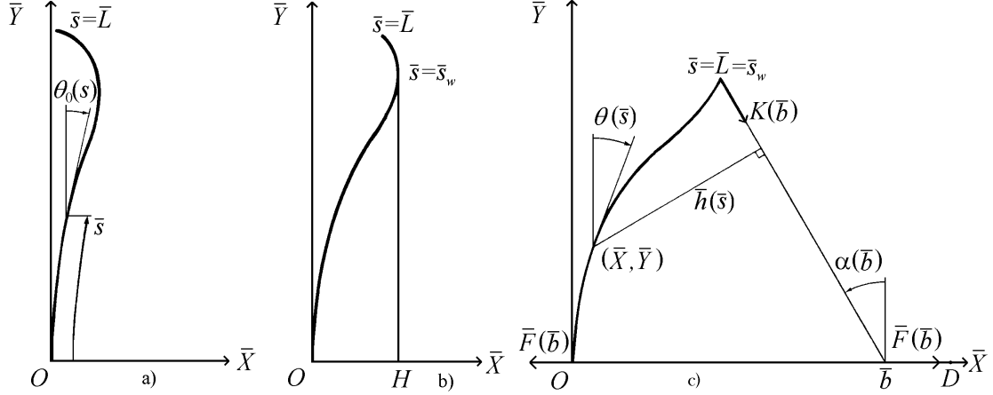
Figure 1: Three situations of the working-recurve bow: a) unbraced, b) braced, c) partly drawn.
