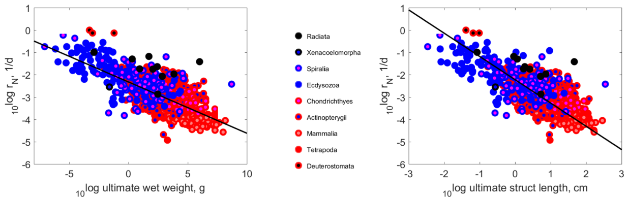
Fig. 2. The specific population growth rate, \dot{r}_N , at 20 °C, as function of predicted maximum body weight (left panel) or structural length (right panel). Thinning is applied if \dot{R}_i > 1 \text{ d}^{-1} . The first principal component is indicated, which has slope -0.23 and -1.09 , respectively. All calculations were performed at f = 1 .
