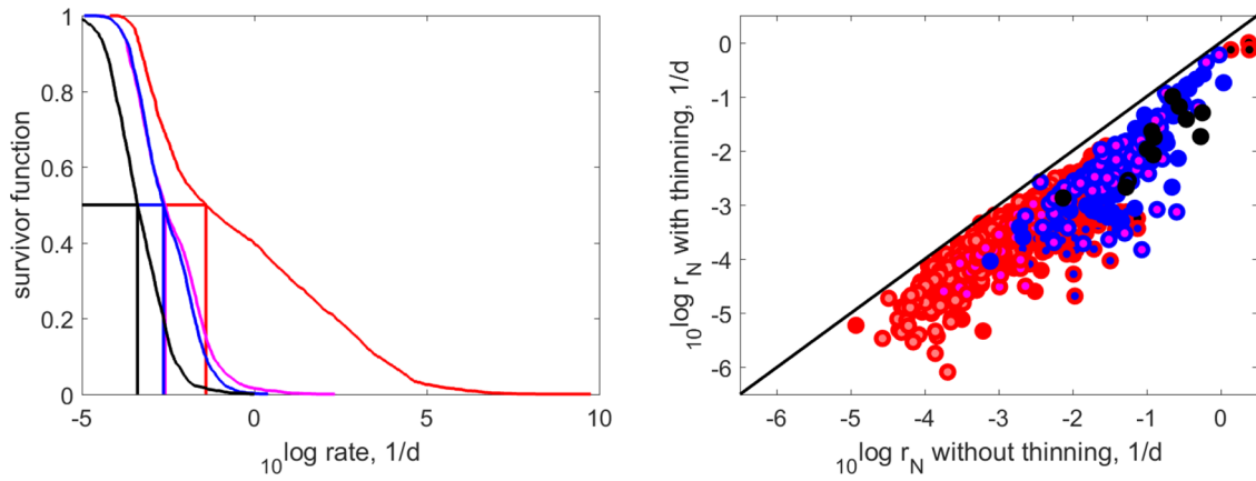
Fig. 1. Left panel: The survivor functions and medians for (from right to left): the maximum reproduction rate \dot{R}_m (red), the ceiling \dot{r}_N^m for the specific population growth rate (magenta), and the specific population growth rate \dot{r}_N without (blue) and with thinning (black), for the 2027 species in the AmP collection (but semelparous species were excluded in \dot{R}_m as such a rate is not defined for them). Right panel: the specific population growth rate \dot{r}_N with thinning, as function of that without thinning. The line of equal rates has been indicated; colour coding as in Fig. 2. All calculations performed at f = 1 and all rates are corrected for 20 °C. (For interpretation of the references to colour in this figure legend, the reader is referred to the web version of this article.)
