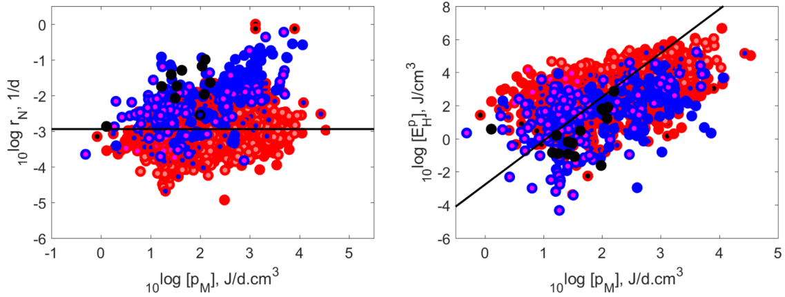
Fig. 4. Left panel: The specific population growth rate, r_N , as function of specific somatic maintenance [p_M] . Thinning is applied if \dot{R}_l > 1 \text{ d}^{-1} . The line is the first principle component with slope 0. Right panel: The specific maturity at puberty, [E_H^p] , as function of [p_M] . The line is the first principle component with slope 2.65. All calculations performed at f = 1 and all rates are corrected for 20^\circ \text{C} ; colour coding as in Fig. 2.
