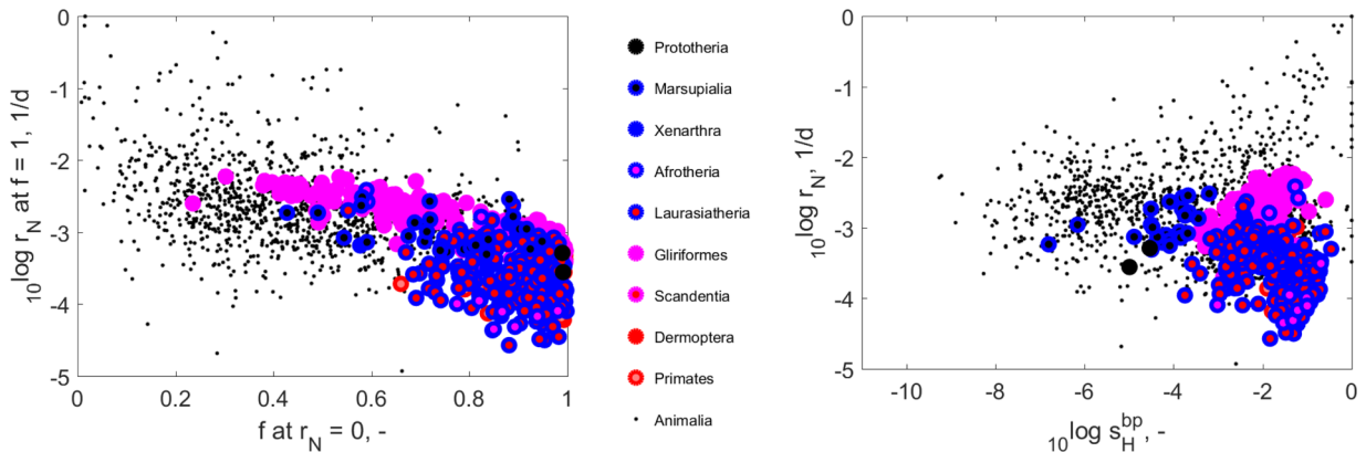
Fig. 5. The specific population growth rate, \dot{r}_N , at 20^\circ \text{C} and abundant food ( f = 1 ), as function of the minimum functional response f_0 (left panel) and of the precociality index s_H^{bp} (right panel). Thinning is applied if \dot{R}_l > 1 \text{ d}^{-1} .
